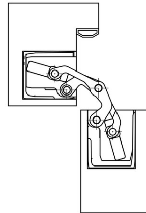
Blockzarge 90°
