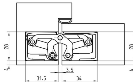
Blockzarge
